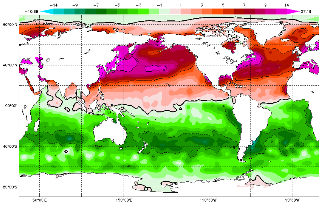
SST_Diff_(Jyly/Aug)-(Jan/Feb)2011
