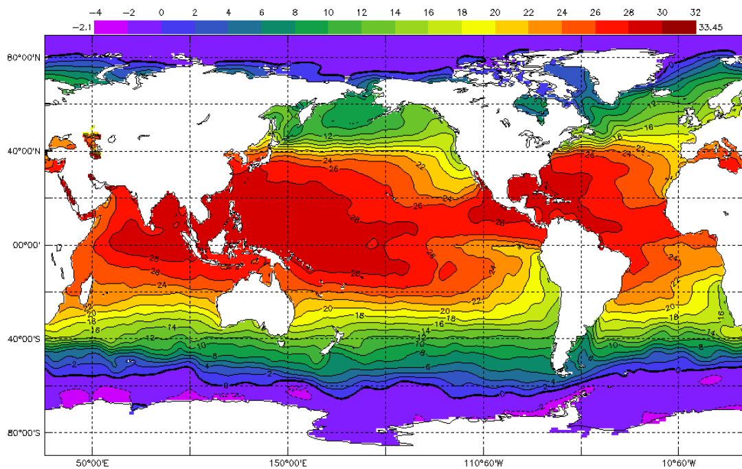
SST_July/Aug2011
